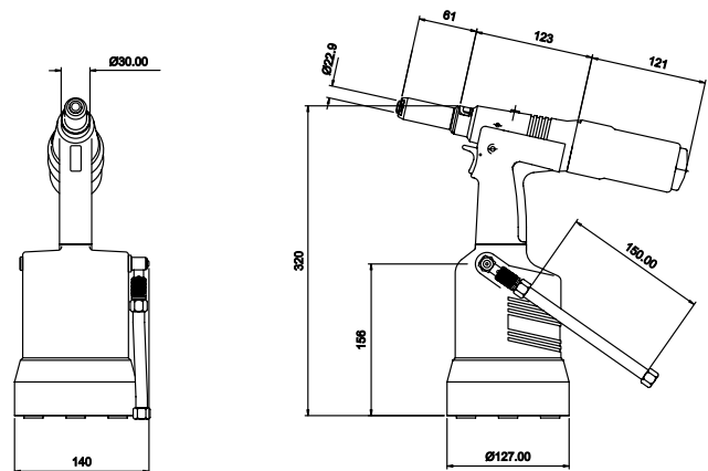
Quick release stem collector bottle option (71233 series)
