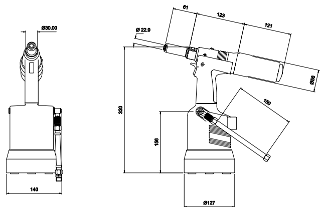
Quick release stem collector bottle option (71223 series)
